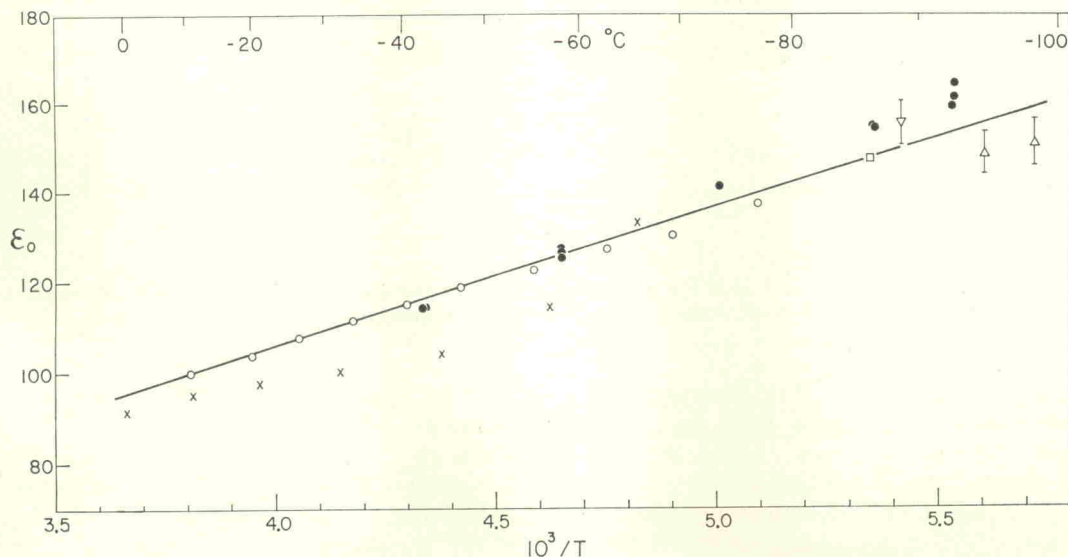
FIG. 5. Static permittivities of hexagonal ice: X, data of Auty and Cole 1 ; O, sample frozen from liquid; otherwise samples prepared from ice II or IX in the coaxial cell.
